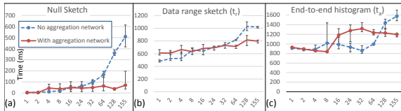
Figure 9: Scale-out experiment, where we keep a constant amount of data per server and increase the number of servers. Graph displays end-to-end time measured at client for computing various sketches. X axis is number of server machines, Y axis is time in milliseconds.
