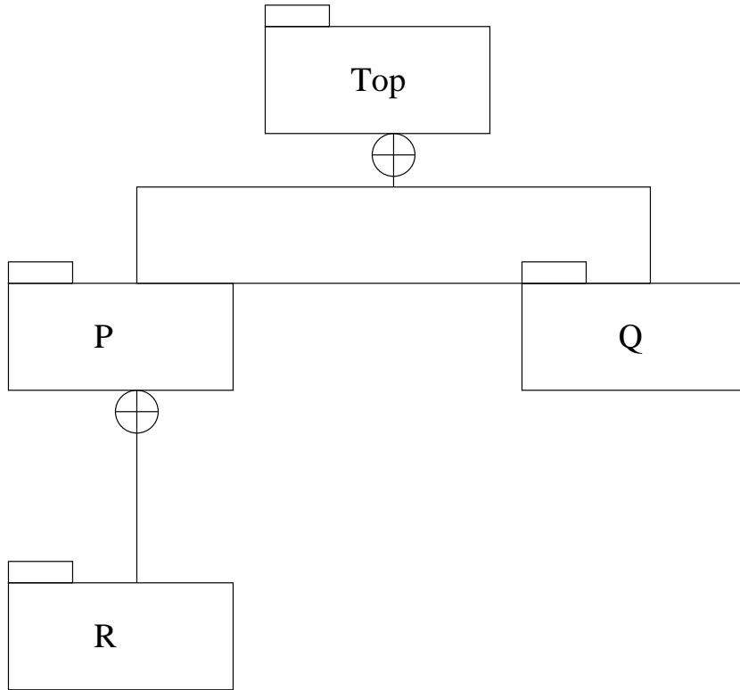
Figure 1: A hierarchy of packages.
