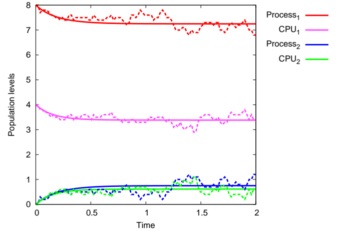
Figure 3: ODE and SSA analysis of the simple PEPA model in Figure 1. Solid lines represent the ODE solution and dotted lines the SSA (performed with 10 independent replications). The legend is ordered by final population level from the ODE solution.
